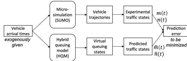
Figure 4: HQM approximates SUMO by tracking the vehicle counts on the highway section.
