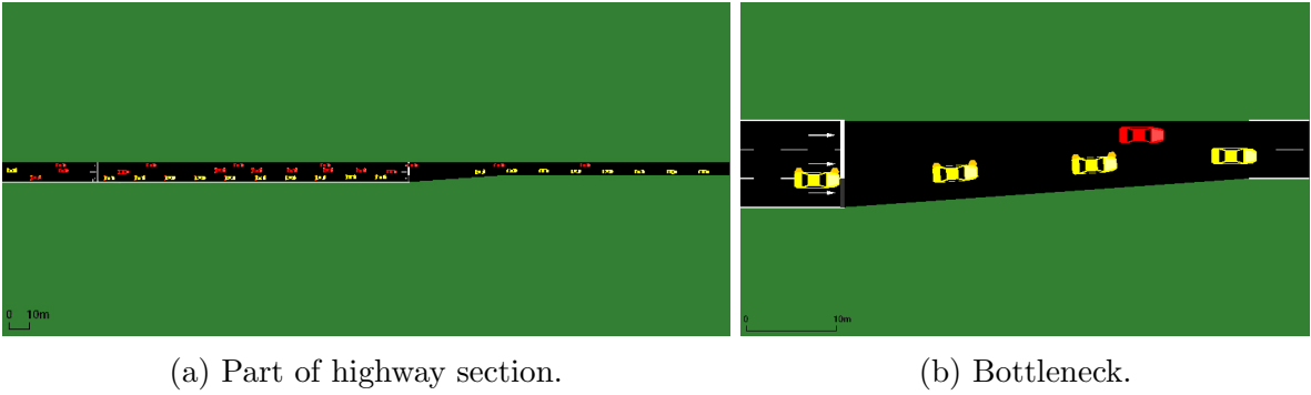
Figure 5: SUMO simulation testbed. Red (resp. yellow) vehicles are non-CAVs (resp. CAVs).
