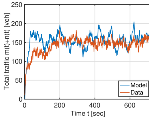
Figure 6: The HQM (“model”) adequately tracks the total vehicle count in SUMO (“data”).
