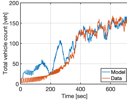
Figure 9: HQM gradually learns and tracks SUMO results.
