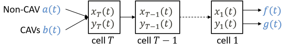
Figure 2: Hybrid queuing model for a highway section.
