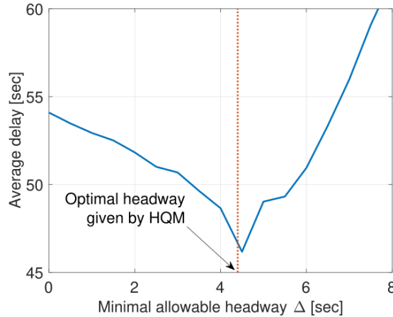
Figure 7: Average delay simulated in SUMO. The HQM gives an optimal headway of 4.4 sec, which is close to the numerical optimum.
